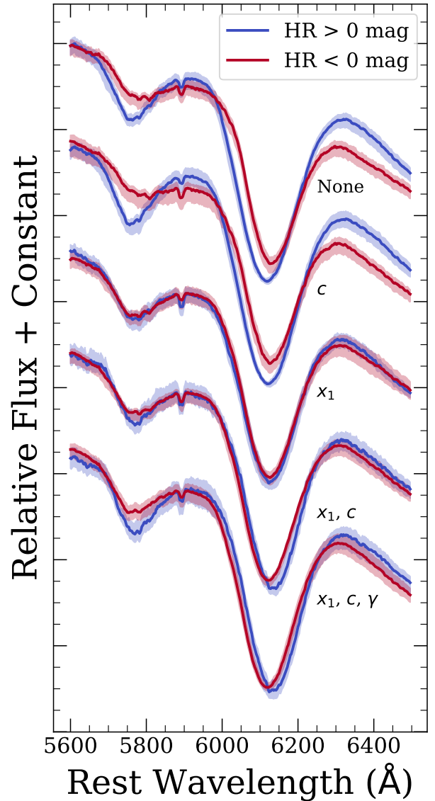
Figure 15. Same as Figure 5 but zoomed in on the Si II \lambda 6355 feature.
