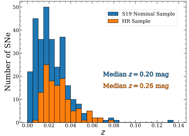
Figure 3. Same as Figure 2, but for redshift.
