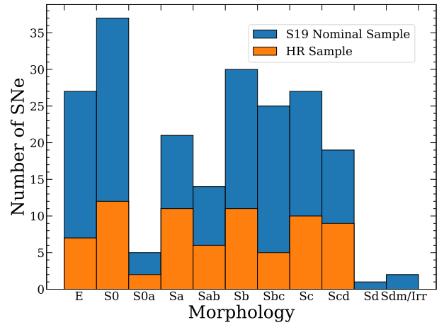
Figure 4. Same as Figure 2, but for host-galaxy morphology.
