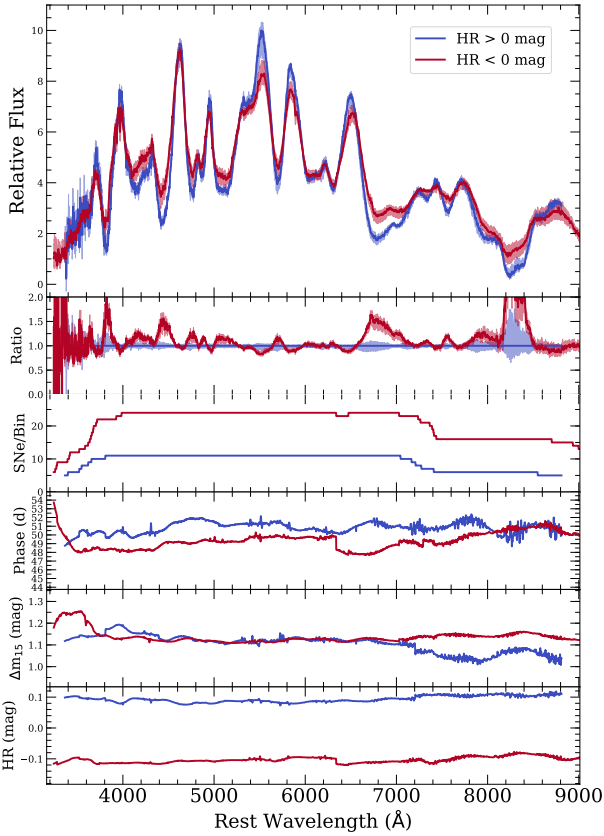
Figure 13. Same as Figure 6 but comparing the +52-day HR-binned composite spectra.
