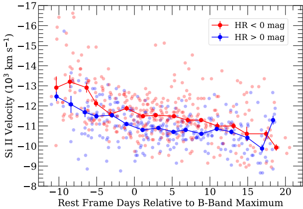
Figure 14. Si II velocity evolution for the HR sample. Individual points are measurements made from individual spectra. Solid connected points are binned medians using the bin sizes of 2 days and the error bars are the median absolute differences, dividing by the square-root of the number of points in a bin, for each bin. Blue and red points correspond to measurements from SNe in the positive-HR and negative-HR samples, respectively. We estimate that the negative-HR sample has a mean velocity that is at least 500 km s -1 larger than the positive-HR sample at the 2.8 \sigma level.
