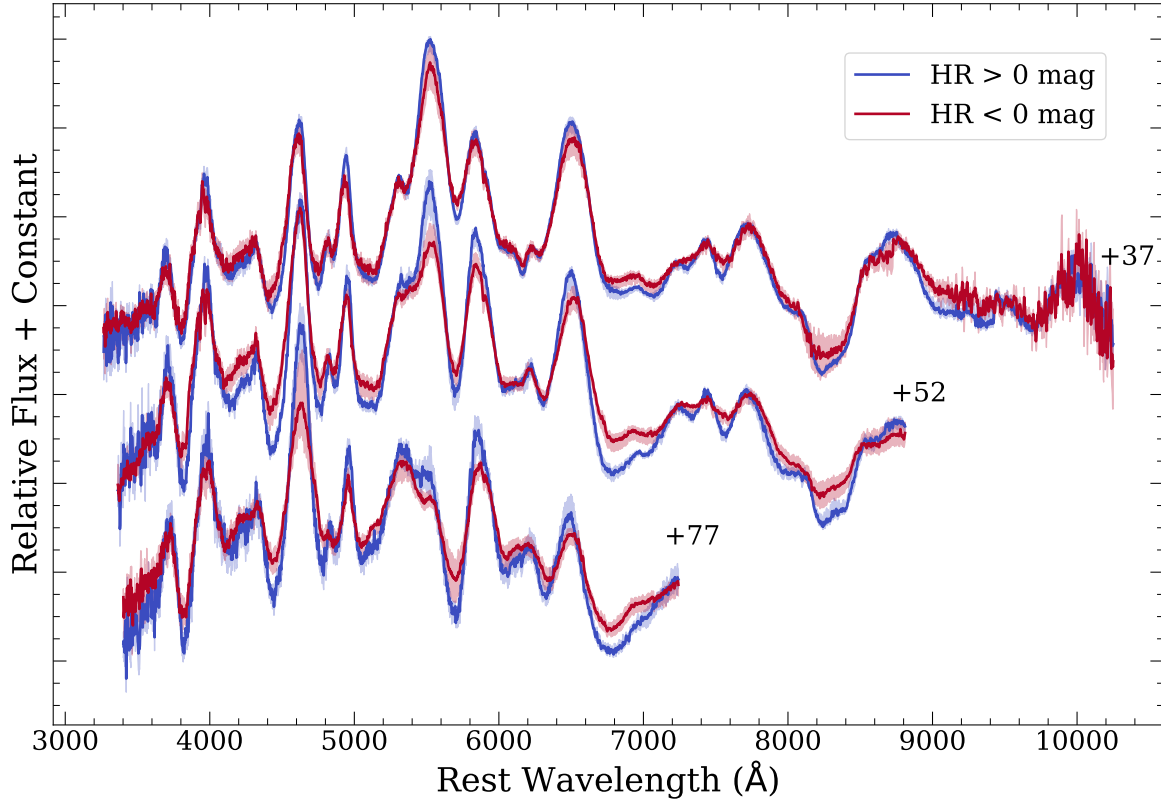
Figure 12. HR-binned composite spectra Composite spectra with effective phases of +37, +52, and +77 days from top to bottom. Blue and red curves/shaded regions correspond to the positive- and negative-HR composite spectra, respectively.
